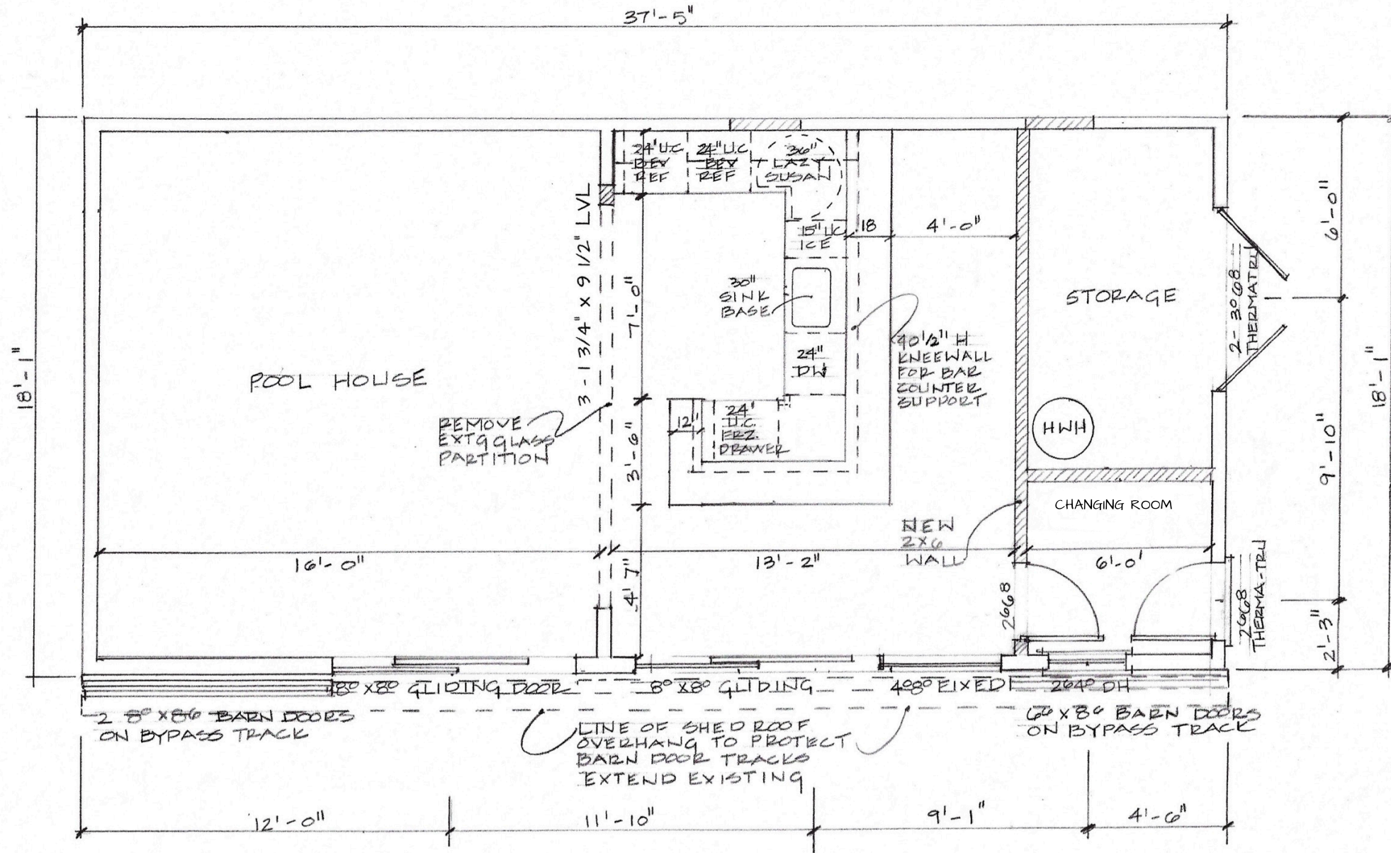
FLOOR PLAN 1/4" = 1'-0"
